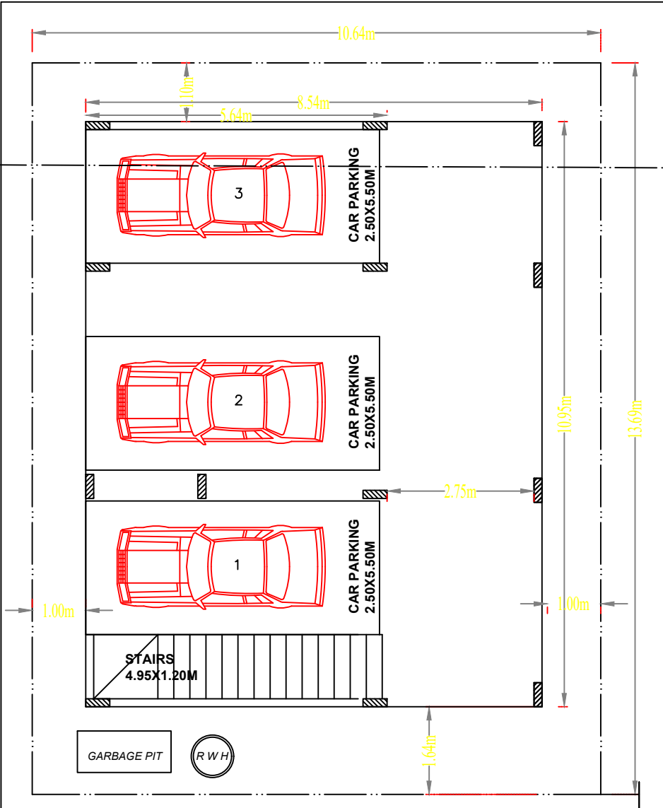
9.00M. WIDE ROAD PROPOSED STILT FLOOR PLAN
